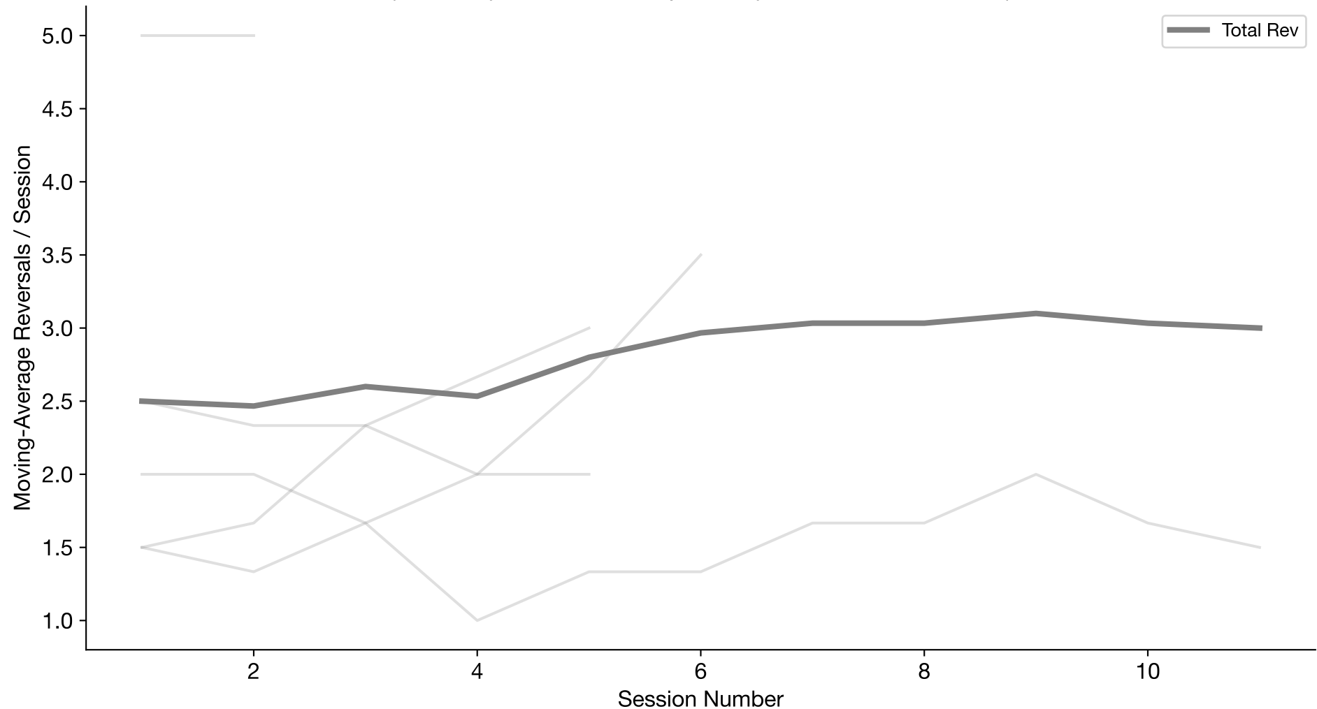
Moving-Average Total Reversals Over Time (n=5 subjects; sessions per subject=2-11; window=3)
